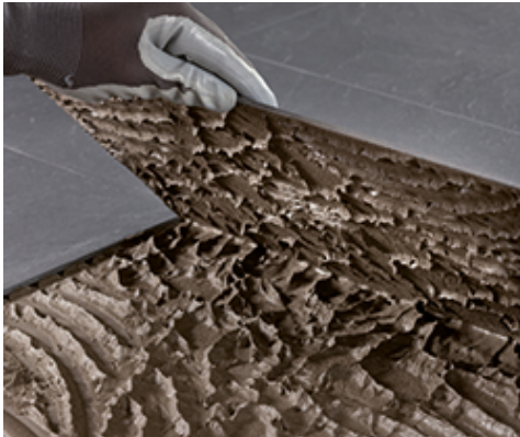
Checking the complete back-buttering of thin porcelain tile
